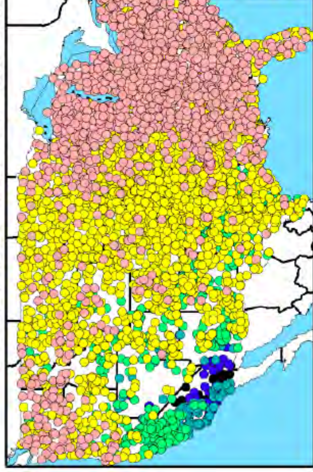
c) AVERAGE NUMBER OF DAYS/YR TO OBTAIN HALF OF TOTAL PRECIPITATION, WY 1951-2008
