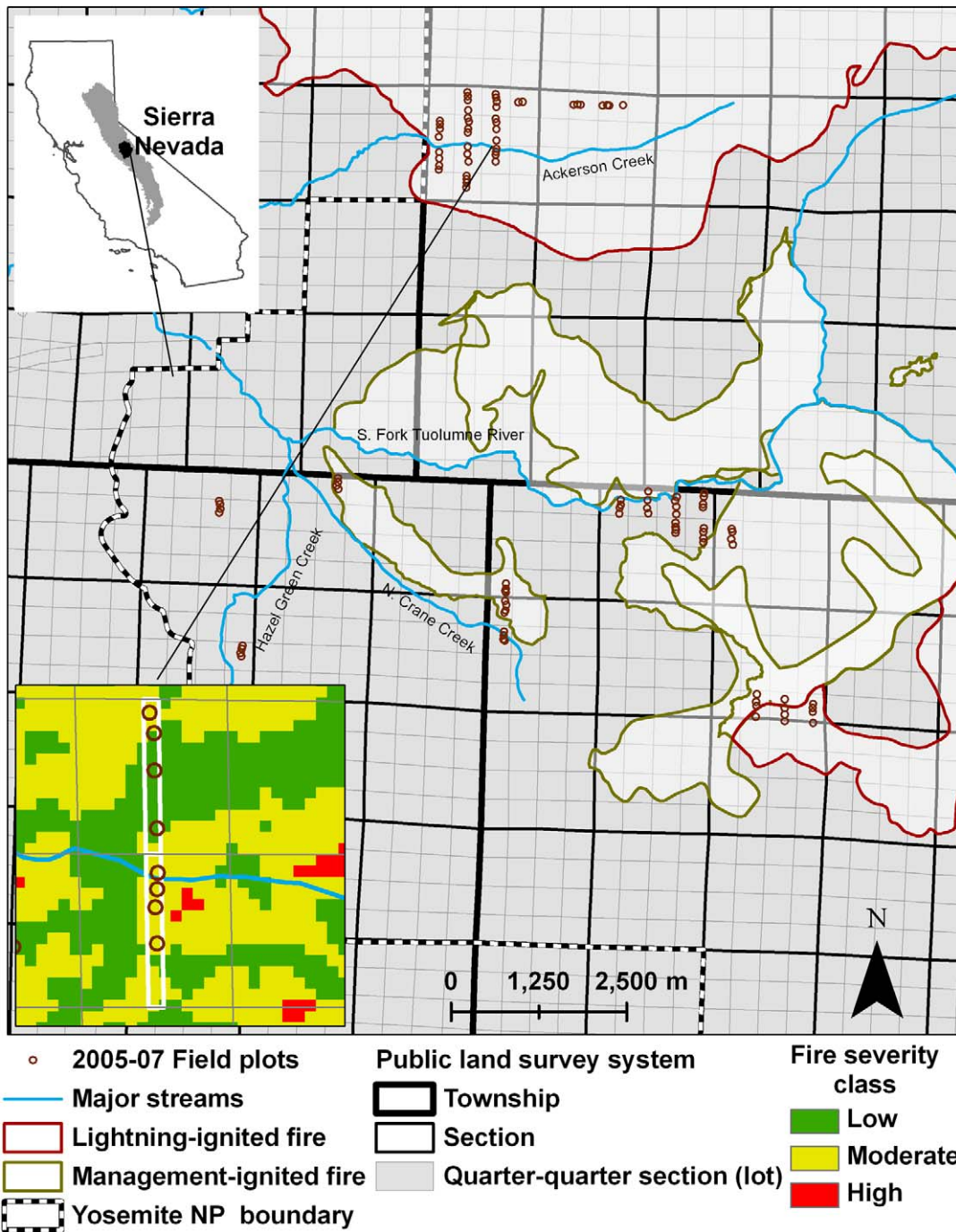
Fig. 1. Locations of lots included in the 1911 timber inventories that were re-sampled between 2005 and 2007 within Yosemite National Park, California, USA. Portions of the study area have burned in seven management- and lightning-ignited fires, occurring between 1983 and 2002. The lower left frame demonstrates both the re-sampling effort within the estimated historical belt transect (white rectangle outline), and the satellite-derived fire severity classification used to broadly capture fire effects on dominant vegetation (see Methods).
