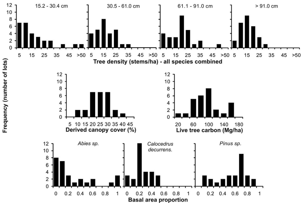
Fig. 3. Frequency distributions of forest structure and composition attributes based on 1911 timber inventories. These attributes were constructed using only live conifers \geq 15.2 cm diameter at breast height (dbh). The size ranges in the upper graphs are for four dbh classes.
