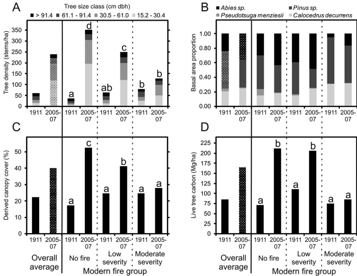
Fig. 2. Average forest structure and composition attributes by sampling period and by modern fire group. These attributes were constructed using only live conifers \geq 15.2 cm diameter at breast height (dbh) and include: tree density (all species combined) by dbh class (A), proportion of basal area by species group (B), derived canopy cover (see Methods) (C), and live tree carbon (D). Dotted bars represent significantly ( P < 0.05 ) higher overall period averages. Letters above bars indicate significantly different period/modern fire groups based on pairwise comparisons using Tukey-Kramer adjusted P -values. Comparisons indicated in (A) are for aggregated tree density (all trees >30.5 cm dbh).
